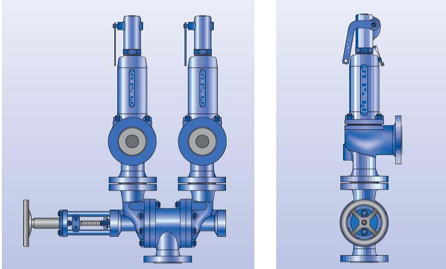
Figure 6.3.6-2: Inlet sided combination
