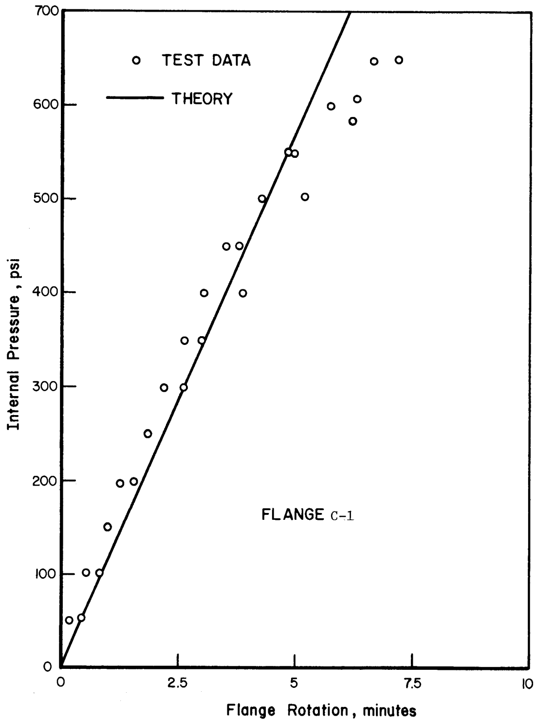
FIGURE A5. COMPARISON OF THEORETICAL AND MEASURED FLANGE ROTATIONS DUE TO INTERNAL PRESSURE, FLANGE C-1, REFERENCE (7) TEST DATA
