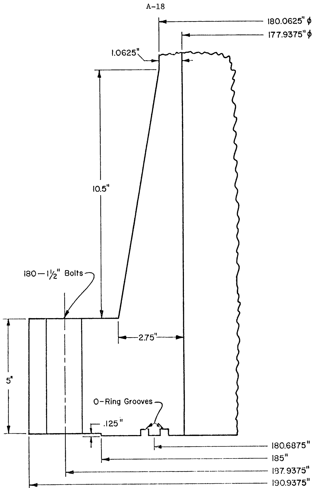
FIGURE A7. DIMENSIONS OF REFERENCE (8) FLANGES, IDENTICAL PAIR USED IN JOINT.
