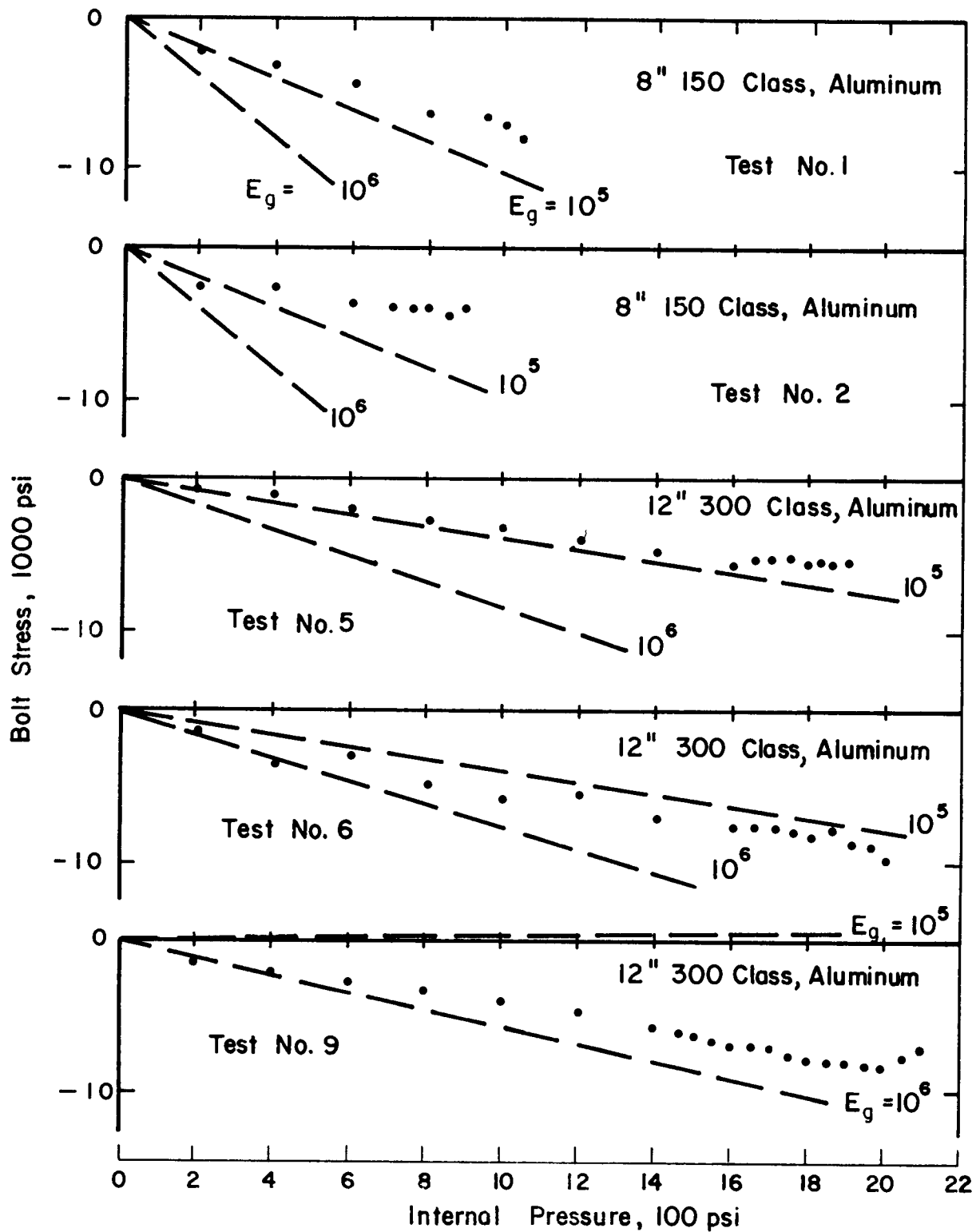
FIGURE A11. COMPARISONS OF THEORETICAL AND MEASURED CHANGE IN BOLT STRESS WITH PRESSURE, REFERENCE (9) TEST DATA.
