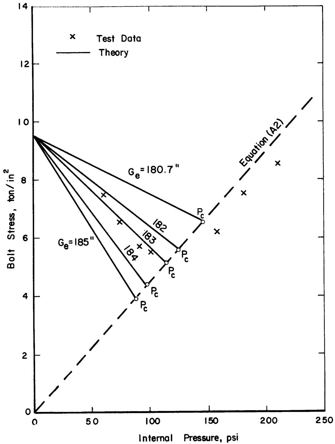
FIGURE A8. COMPARISON OF THEORETICAL AND MEASURED CHANGE IN BOLT STRESS WITH PRESSURE, REFERENCE (8) TEST DATA.
