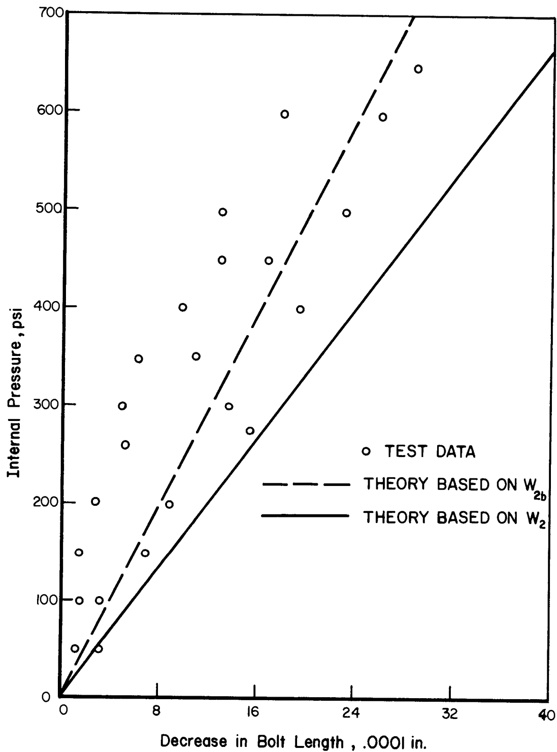
FIGURE A2. COMPARISON OF THEORETICAL AND MEASURED CHANGE IN BOLT LENGTH WITH PRESSURE, REFERENCE (7) TEST DATA.
