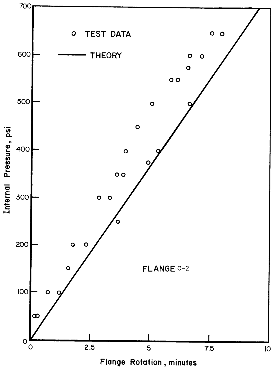
FIGURE A6. COMPARISON OF THEORETICAL AND MEASURED FLANGE ROTATIONS DUE TO INTERNAL PRESSURE, FLANGE C-2, REFERENCE (7) TEST DATA
