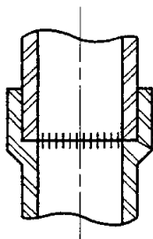
Socket Joint
