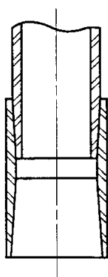
FIG. A328.5.6 FULLY TAPERED THERMOSETTING ADHESIVE JOINT
