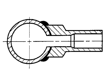
Saddle Joint
