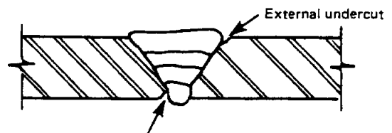
Internal undercut
