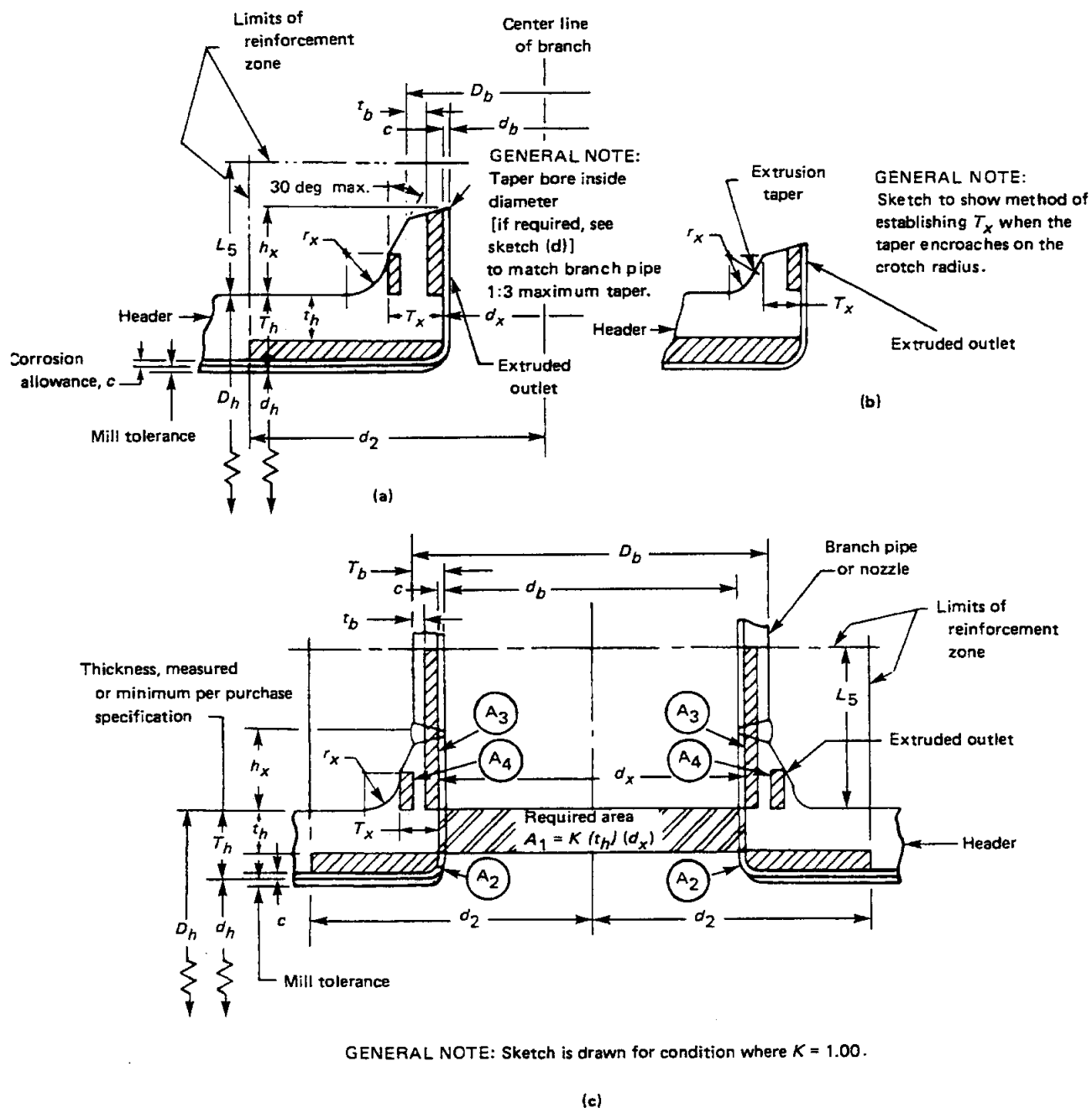
FIG. 304.3.4 EXTRUDED OUTLET HEADER NOMENCLATURE This Figure illustrates the nomenclature of para. 304.3.4. It does not indicate complete details or a preferred method of construction.
