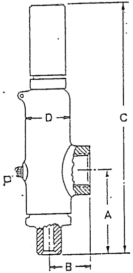
Screwed
